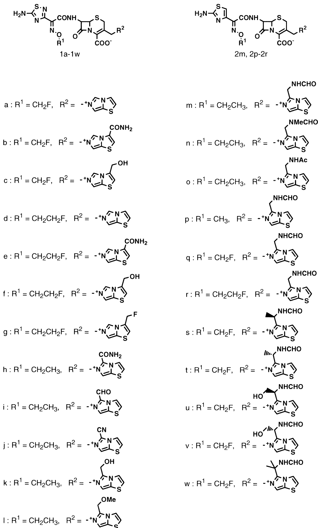
Figure 1. CP6679 (1s) and related compounds.
